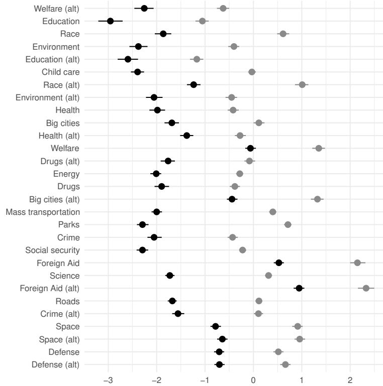
Figure A.13: Estimated cutpoints, 2014 GSS with Alternate Wordings
