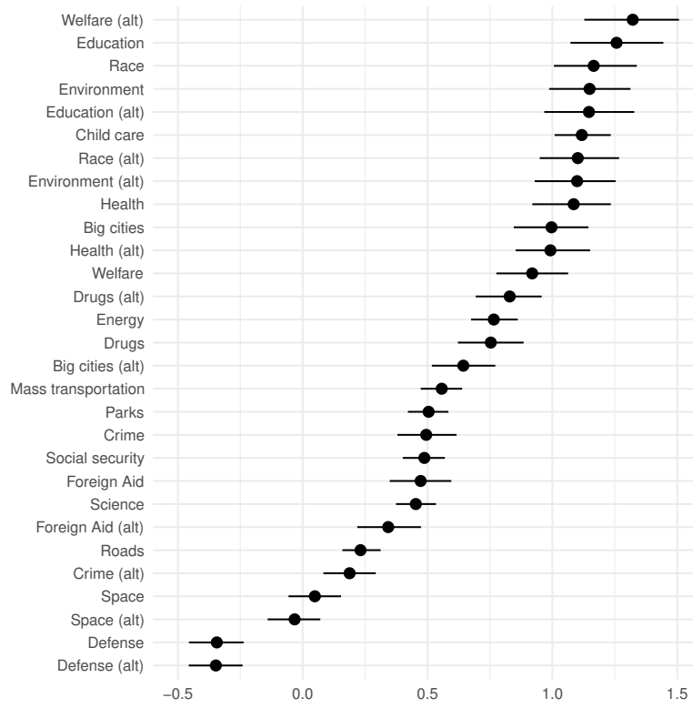
Figure A.12: Discrimination Parameter Estimates, 2014 GSS with Alternate Wordings
