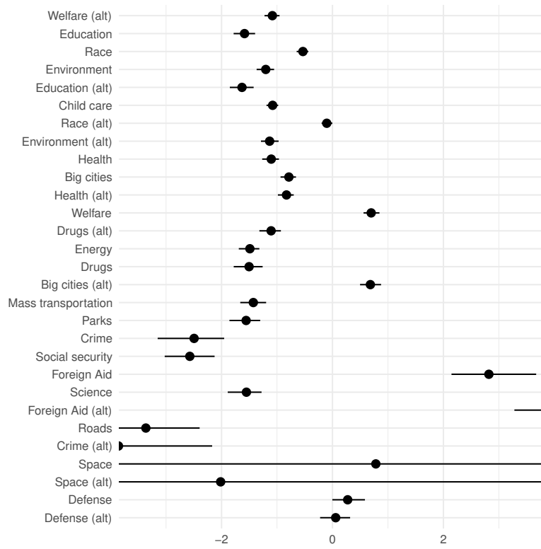
Figure A.14: Ideal Point and Policy Position Estimates, 2014 GSS with Alternate Wordings
